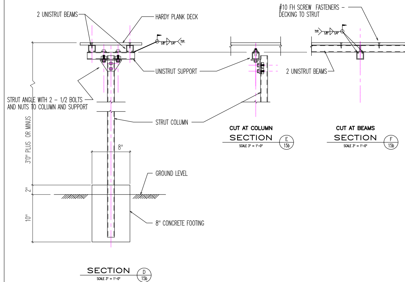
BOLTED / WELDED TOGETHER STRUT ASSEMBLY 15b
