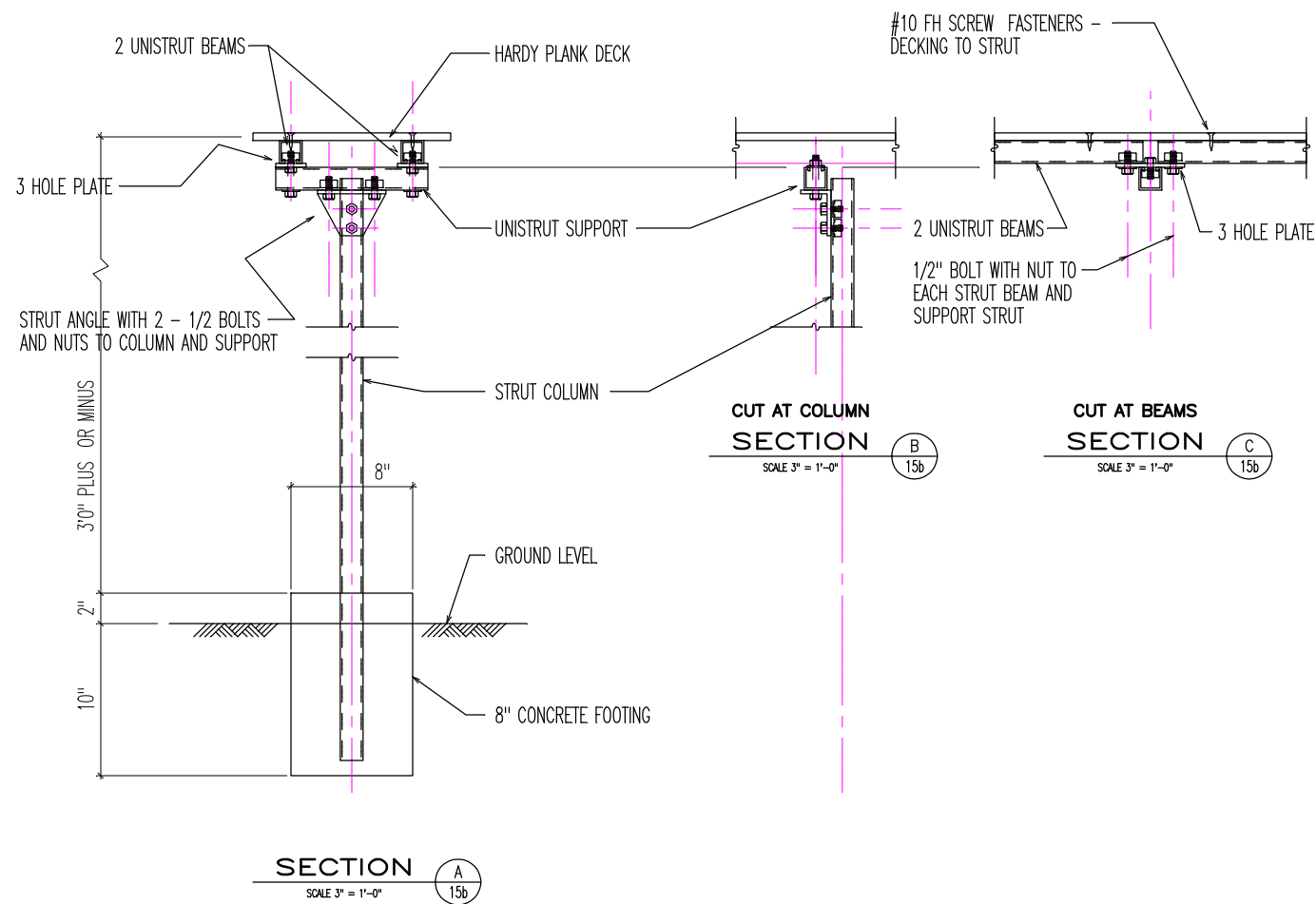
BOLTED TOGETHER STRUT ASSEMBLY 15b
